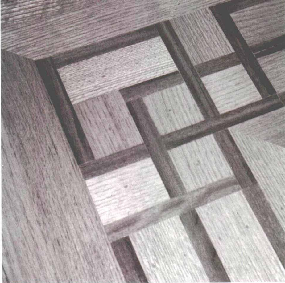
The decorative inlay shown above, a Greek key, is built up as the floor is laid. The inlay is the same thickness as the surrounding flooring. In the photo below, walnut inlay is shown framing a full-room border.
